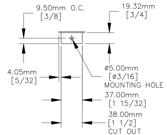
RIGHT VIEW
