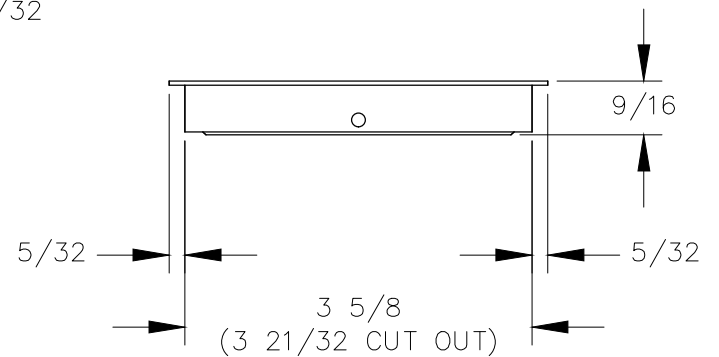
RIGHT VIEW
