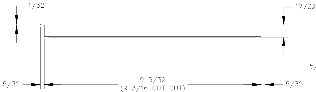
FRONT VIEW
