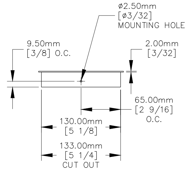
RIGHT VIEW
