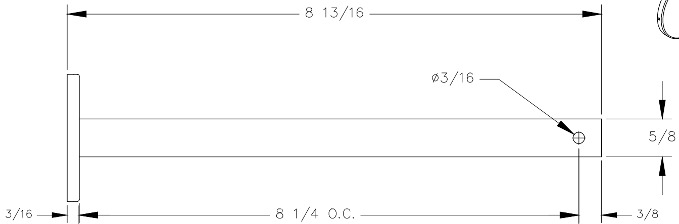
TOP VIEW
