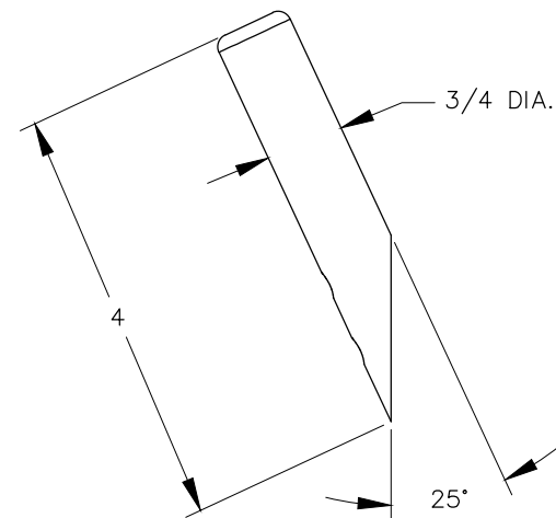
RIGHT VIEW
