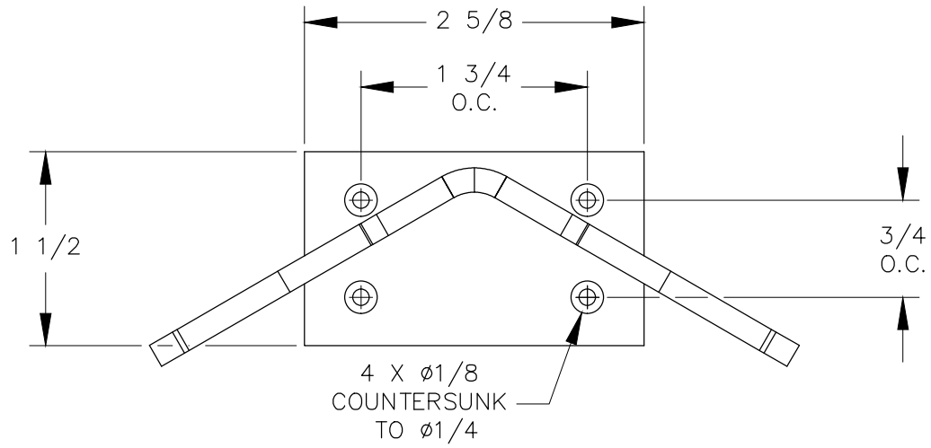
BOTTOM VIEW
