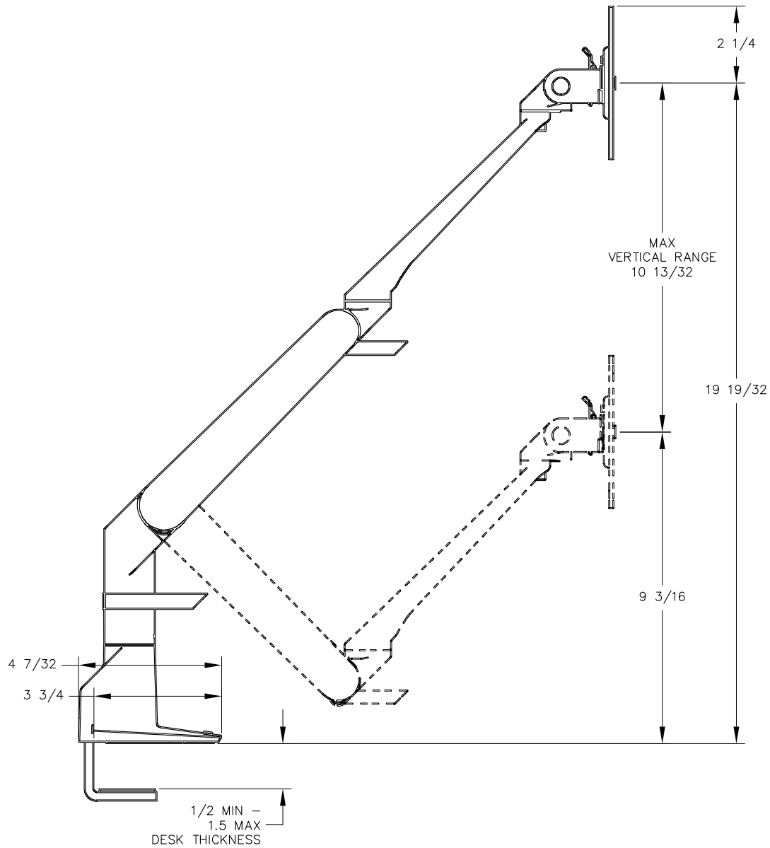
SIDE VIEW
