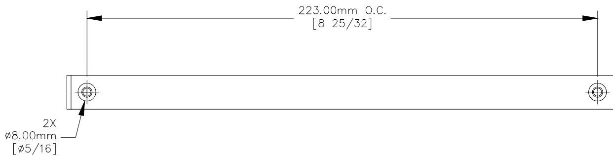
REAR VIEW
