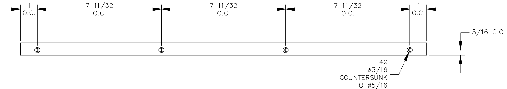
REAR VIEW
