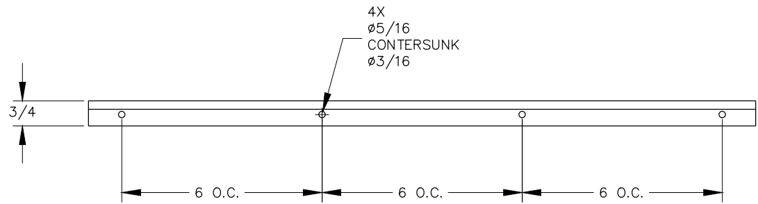
FRONT VIEW
