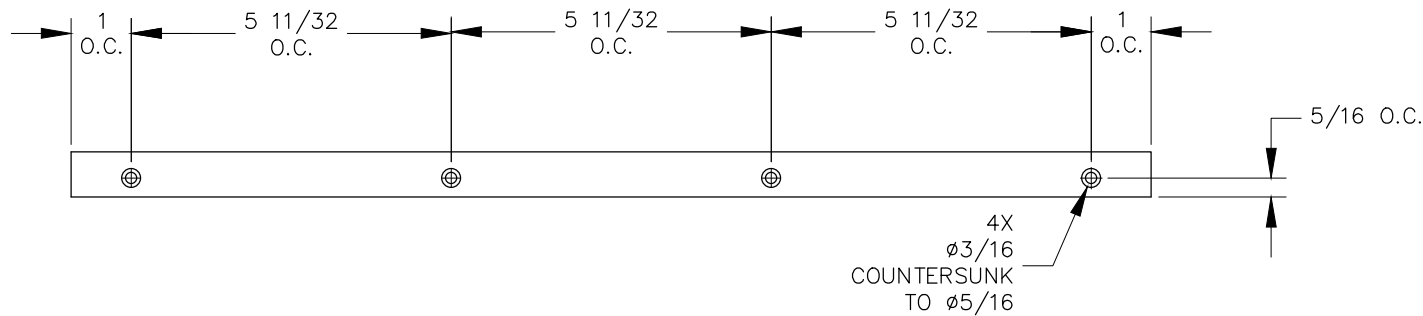
REAR VIEW
