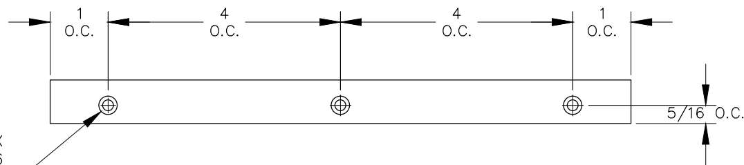
FRONT VIEW
