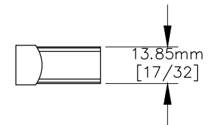
RIGHT VIEW
