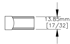
RIGHT VIEW
