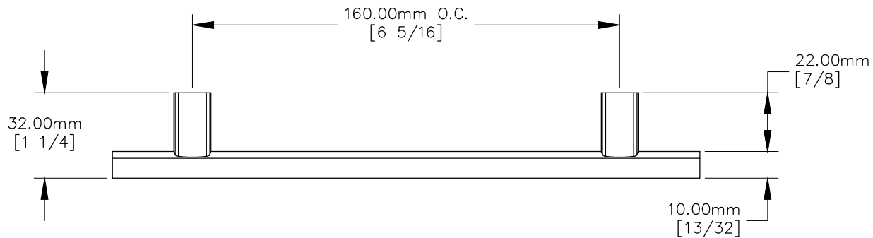
TOP VIEW
