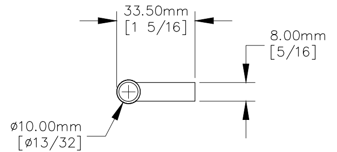
LEFT VIEW
