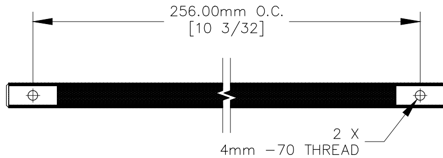
REAR VIEW
