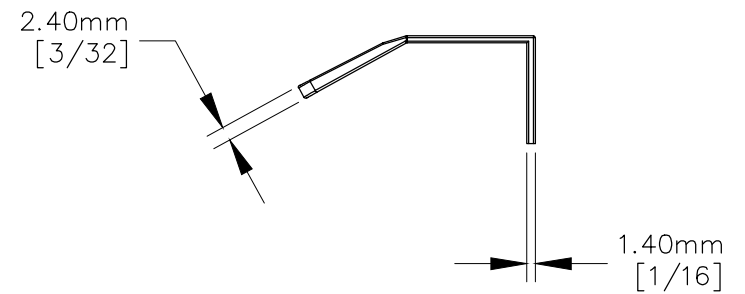
RIGHT VIEW
