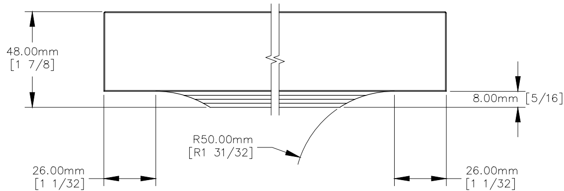
REAR VIEW
