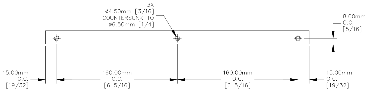
REAR VIEW
