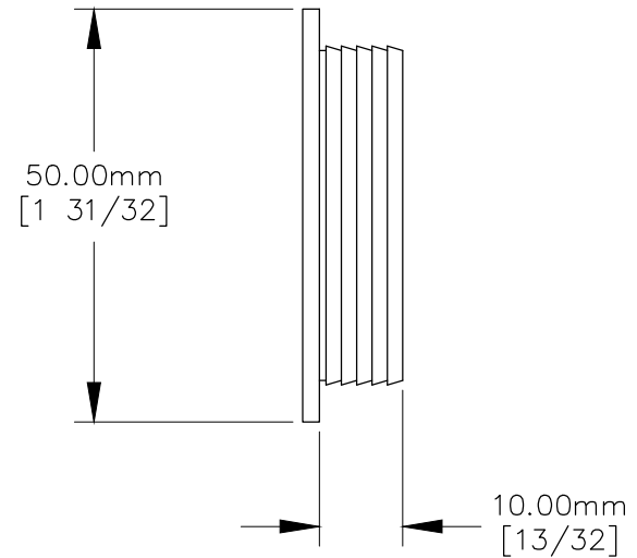
SIDE VIEW
