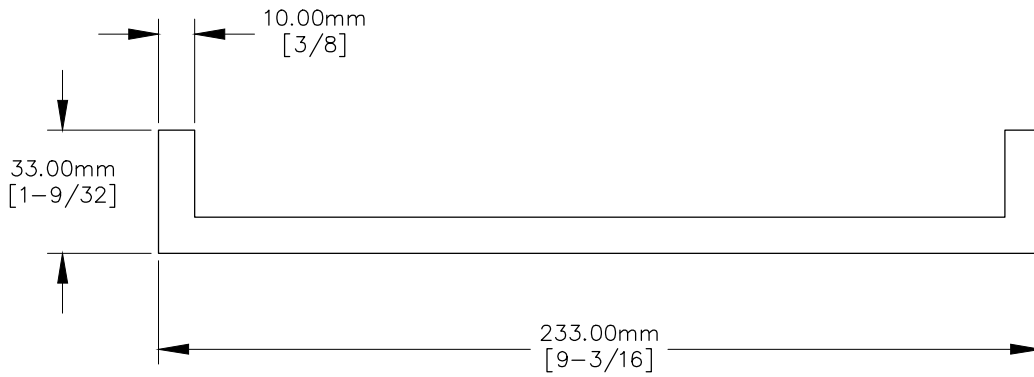
TOP VIEW
