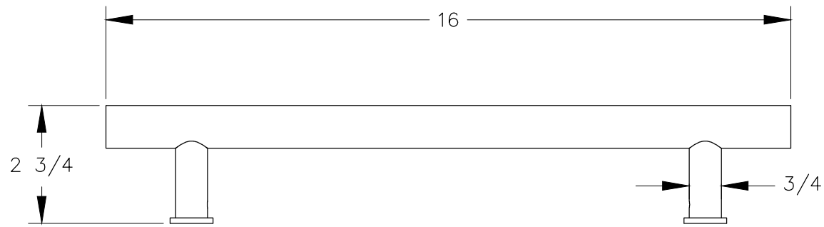
TOP VIEW
