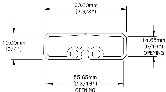
TOP VIEW WM39/LINK
