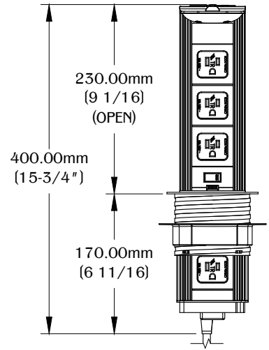
FRONT VIEW (OPEN)
