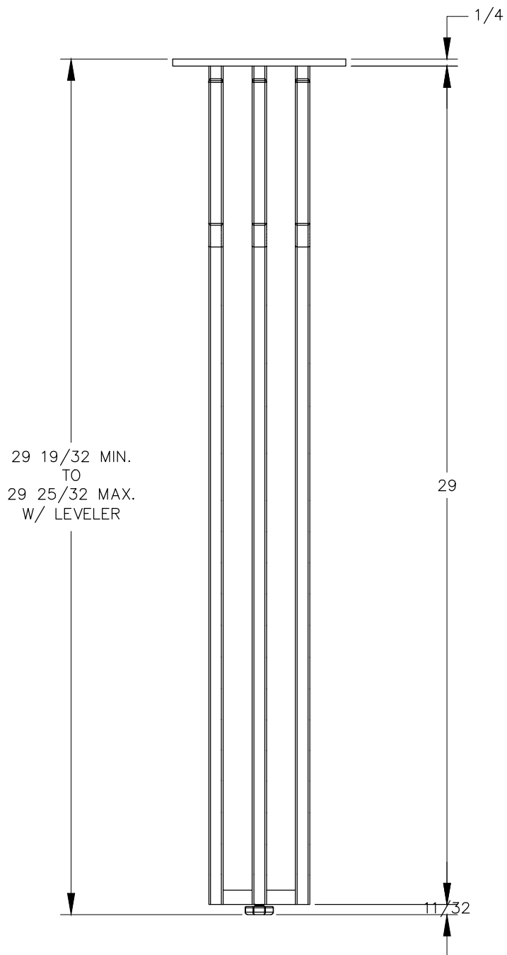
FRONT VIEW
