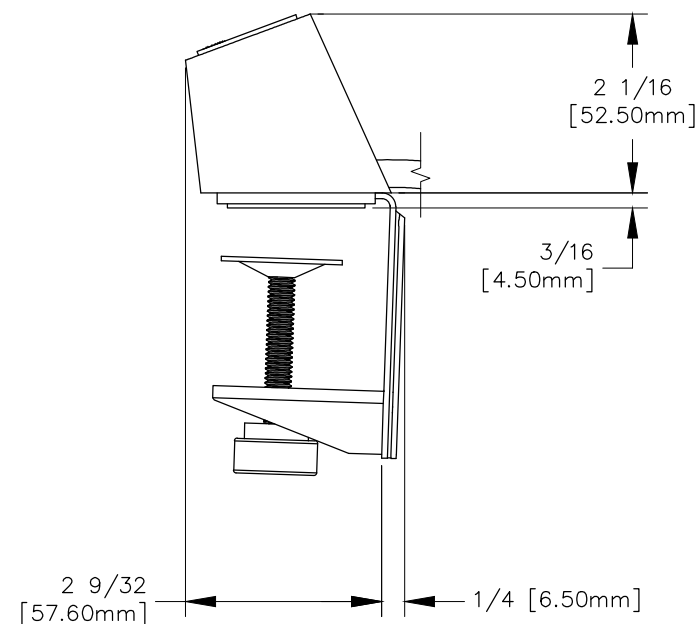
RIGHT VIEW
