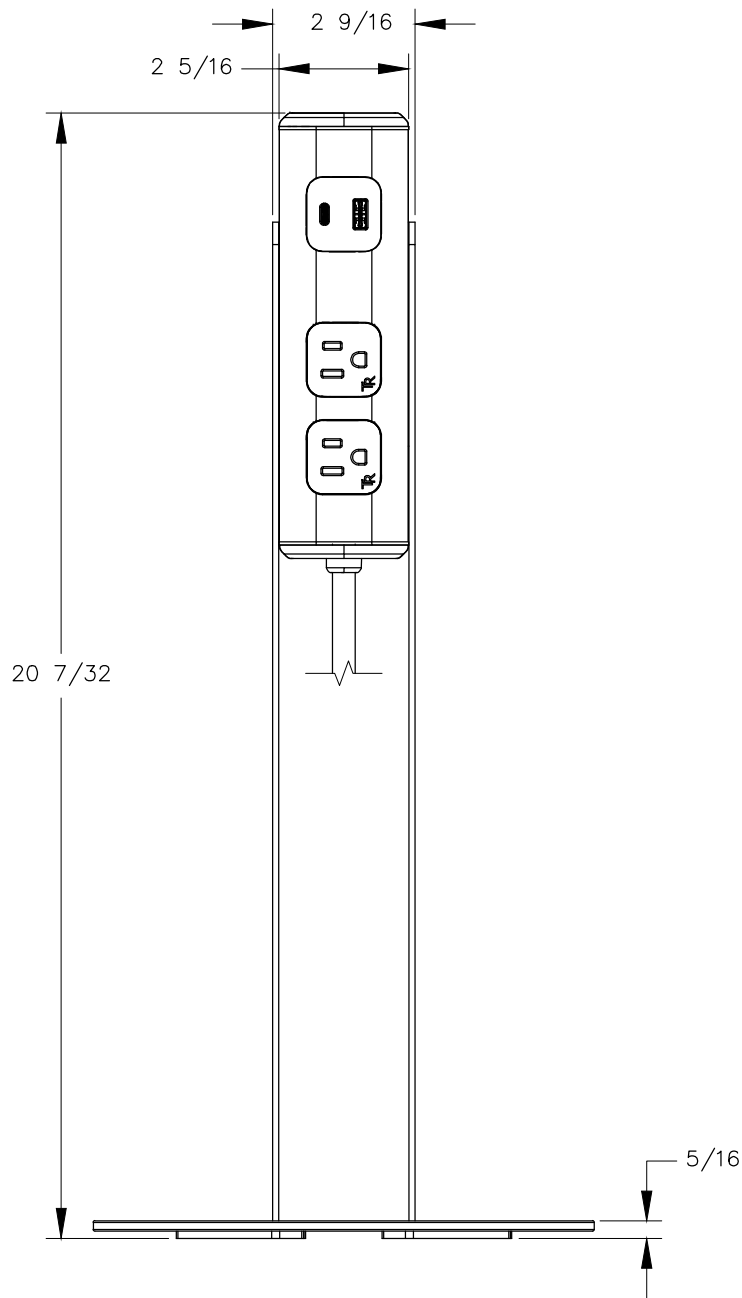
FRONT VIEW
