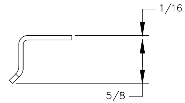
RIGHT VIEW
