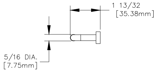
RIGHT VIEW
