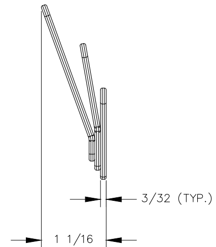
RIGHT VIEW
