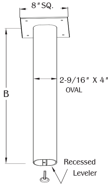
1" Adjustment
